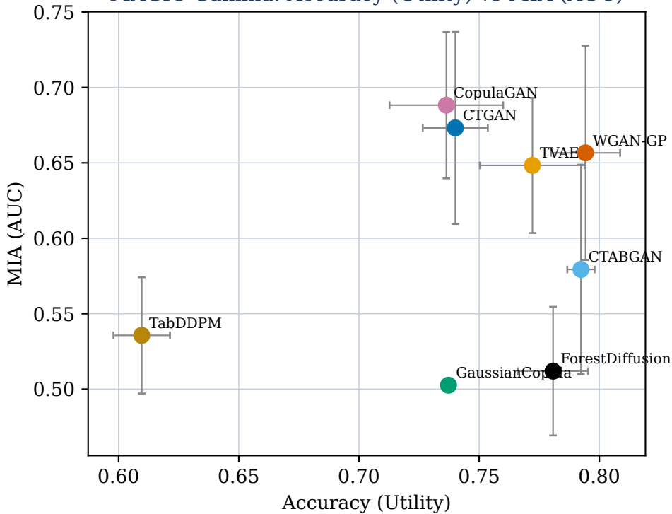
MAGIC Gamma: Accuracy (Utility) vs MIA (AUC)
